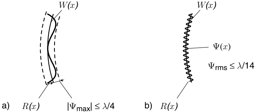
Figure 2.6: Illustration of a) the Rayleigh criterion and b) the Maréchal criterion for the tolerable amount of wavefront aberrations.
