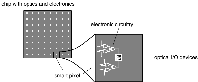
Figure 9.14: Schematic of a smart pixel array consisting of individual devices with optical I/O windows and local electronic circuitry (“smartness”).
