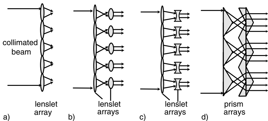
Figure 10.8: Various configurations for multiple beam-splitting through aperture division: a) focusing through a lenslet array; b) Kepler telescope array using two arrays of positive lenses; c) Galilean telescope using arrays of positive and negative lenses; d) anamorphic Brewster telescopes using prism arrays.
