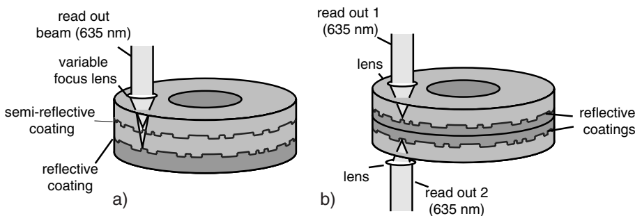
Figure 12.19: Optical data storage in the digital versatile disc: a) multimedia compact disc (Sony/Philips); b) super density disc (Toshiba/Time Warner)
