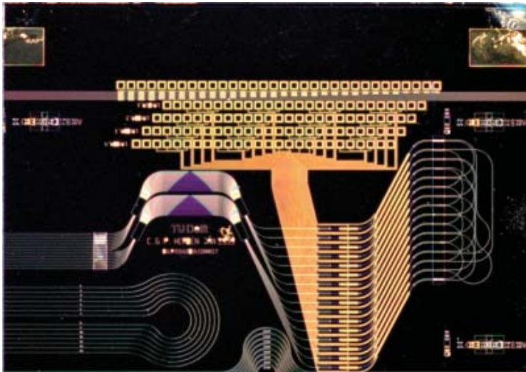
Figure 7.15: The picture shows an InP-based integrated 2x2 WDM crossconnect with four wavelength channels per input/output port. The chip contains two 8x8 PHASAR's for splitting and combining the wavelengths and 16 optical switches from the Mach-Zehnder Interferometer type in a dilated configuration for switching each wavelength individually between the two output ports. Total chip size is 8 \times 12 \text{ mm}^2 (photograph courtesy of M. K. Smit, TU Delft, The Netherlands).
