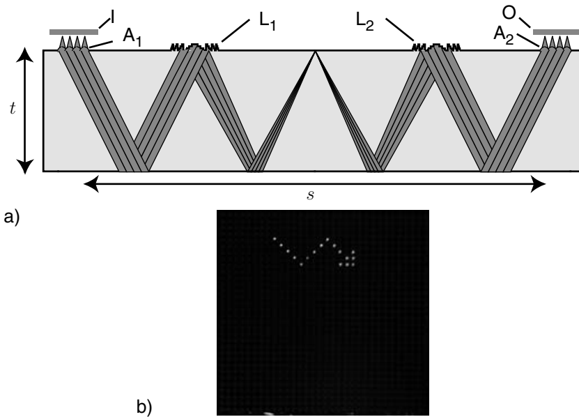
Figure 8.13: a) Schematic of a hybrid imaging system integrated in planar optics (I, O: input and output plane; A_1, A_2 : microlens arrays; L_1, L_2 imaging lenses); b) multiple exposure of the output plane, with different channels “switched on”.
