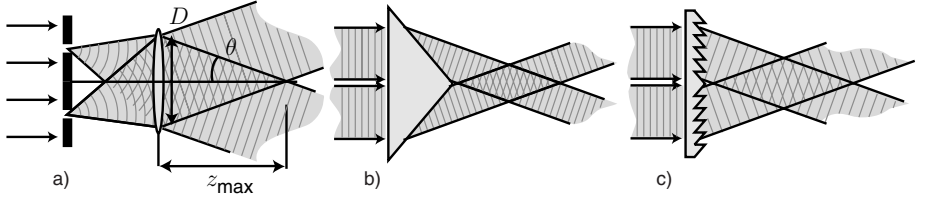
Figure 11.8: Optical setups for generating Bessel beams: a) annular ring aperture followed by a lens; b) classical refractive axicon; c) blazed diffractive axicon. (All elements are circularly symmetric but are shown in crosssection here.)
