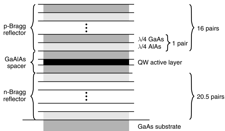
Figure 9.7: Schematic layer structure of a AlGaAs/GaAs VCSEL [17].
