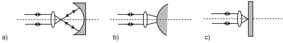
Figure 4.5: Various configurations for null testing of microlenses in a reflection type interferometer using: a) concave, b) convex mirrors, or c) any type of mirror in the cat's eye position.
