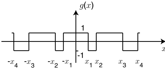
Figure 10.12: Phase profile of one period of a Dammmann grating.
