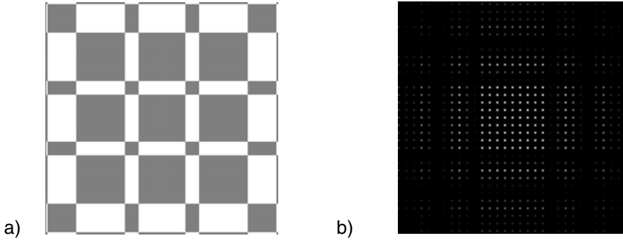
Figure 10.11: Dammmann grating: a) Schematic of one period of a 2D Dammmann grating; b) simulation of the diffraction plane of the Dammmann grating with a 9 \times 9 array of equal intensity diffraction orders. The pictures were generated with the design and simulation tool DIGIOPT [33].
