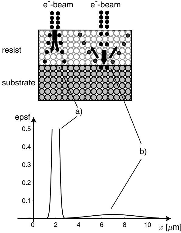
Figure 3.4: Electron scatterings responsible for the proximity effect and their effect on the epsf for typical values of \sigma_f = 0.3 and \sigma_b = 2.8 ; a) elastic forward scattering of the electrons in the resist layer; b) backscattering of secondary electrons generated in the substrate.
