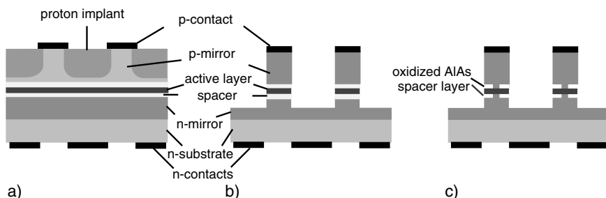
Figure 9.8: Mechanisms for optical and electrical confinement in VCSELs: a) gain-guided resonator; b) index-guided resonator; c) index-guided resonator with oxide confinement.
